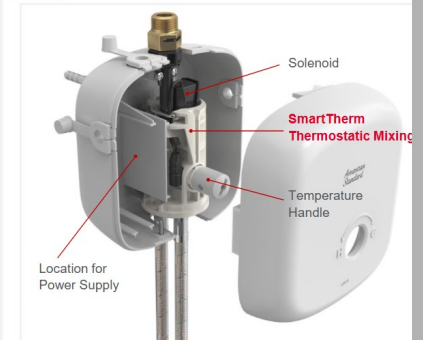
Serin Wall Mount
